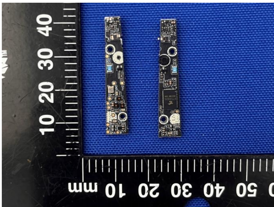
Photo 6: PCB view
