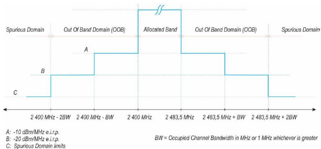
Figure 3: Transmit mask
